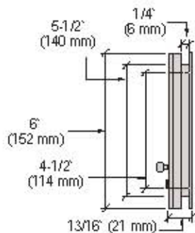
6" (152 mm) Model Requires 5-1/2" (140 mm) Hole
