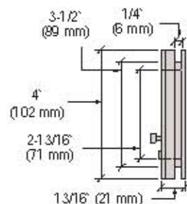
4" (102 mm) Model Requires 3-1/2" (89 mm) Hole
