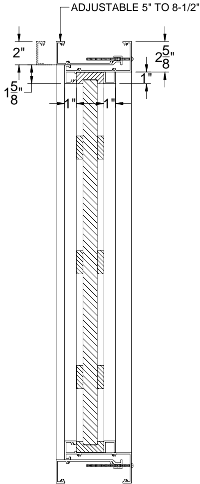
VERTICAL SECTION
