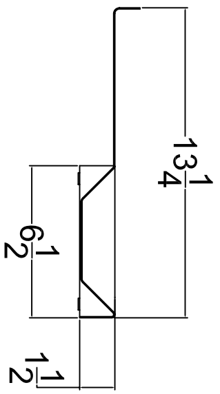
SECTION SLIDING CASH TRAY
